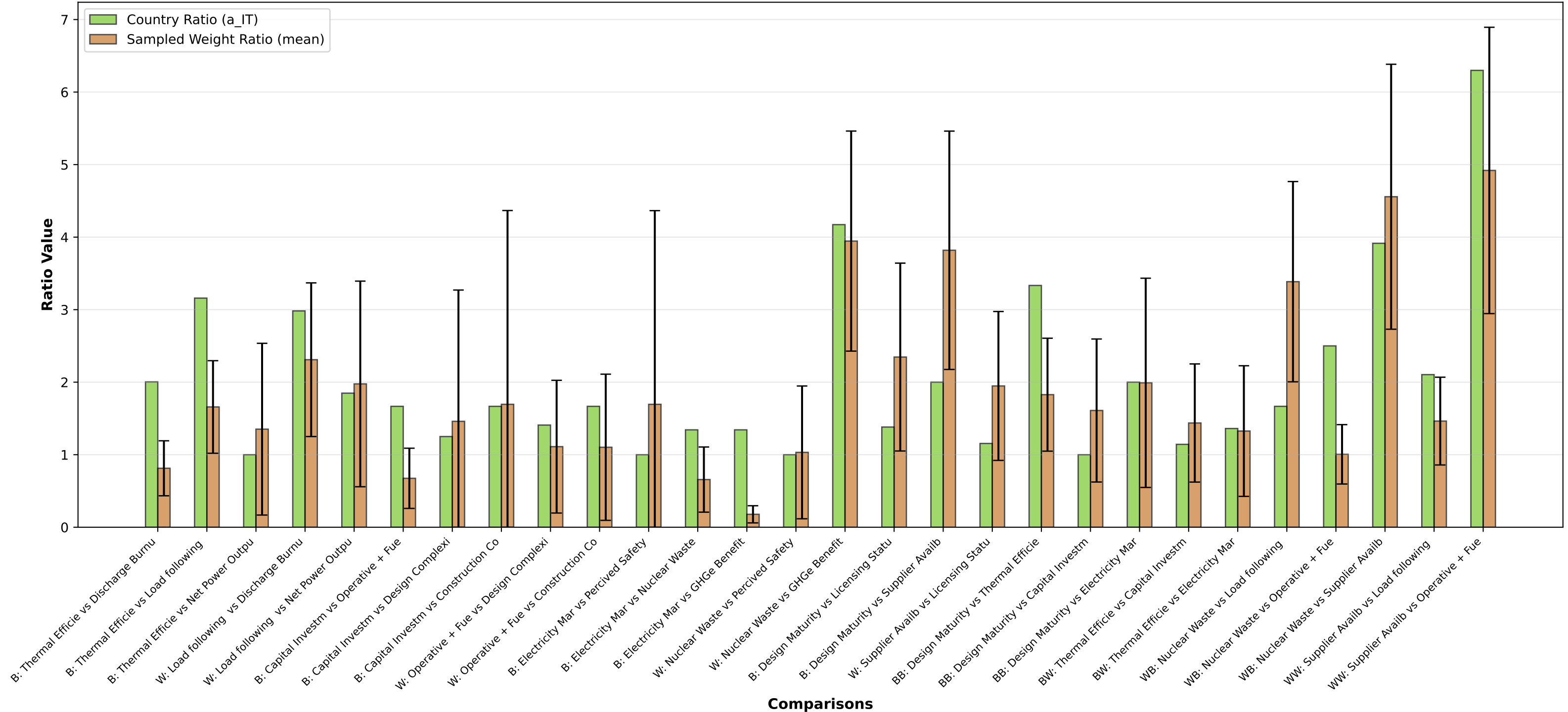
Country vs Sampled Weight Ratios (mean \pm \sigma ) - Elicitation 2 (IT)
